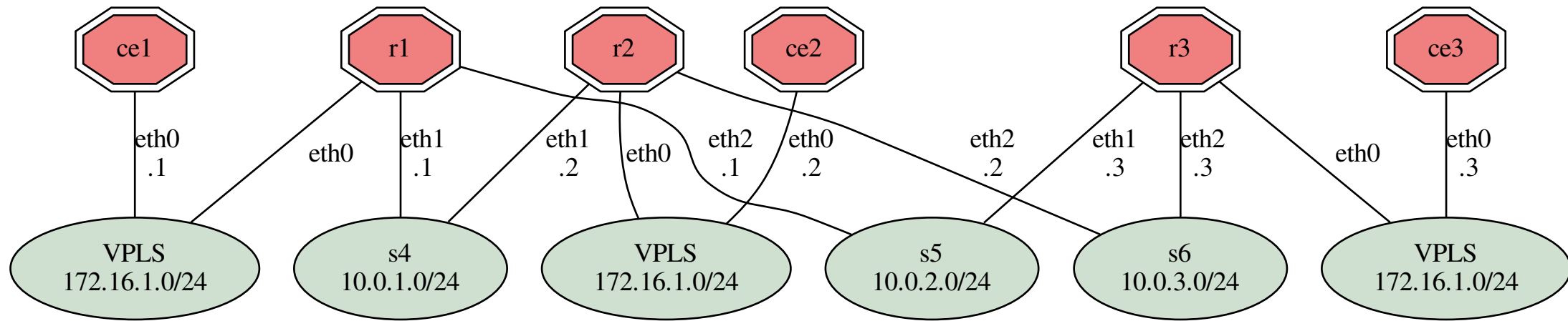
Test Topology - LDP-VPLS 1
